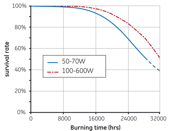
Lamp survival of 50-70W and 100-600W HPS lamps
